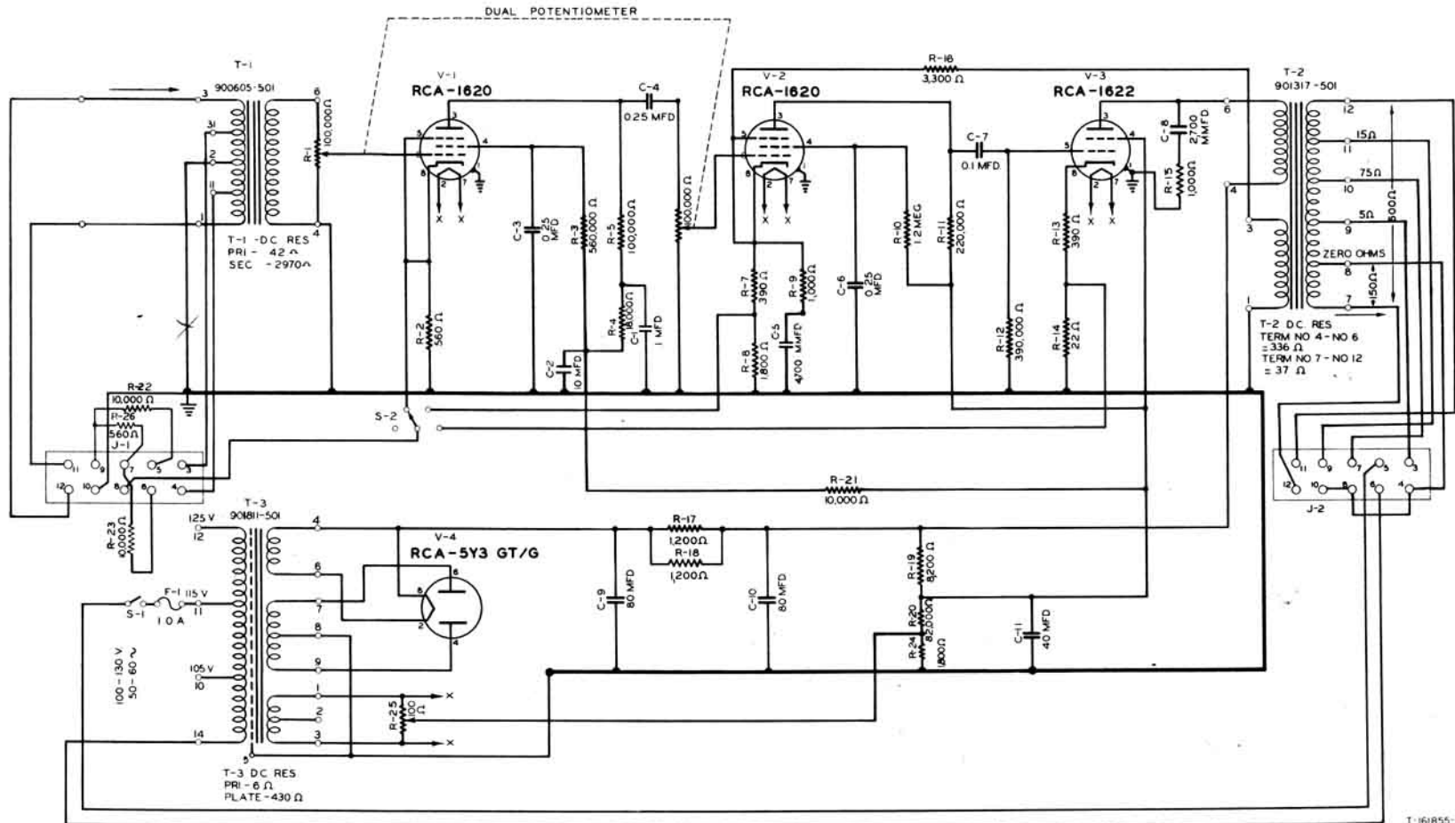
Figure 2—Schematic diagram of Type BA-3C Program Amplifier.
